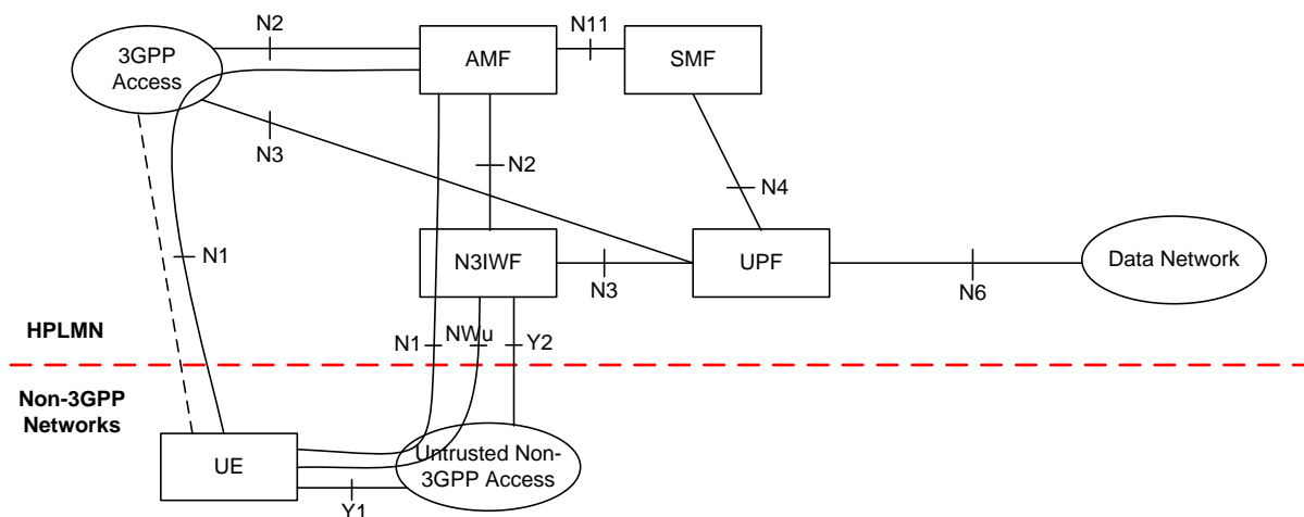
Figure 1: Non-roaming architecture for 5G CN with untrusted non-3GPP access
