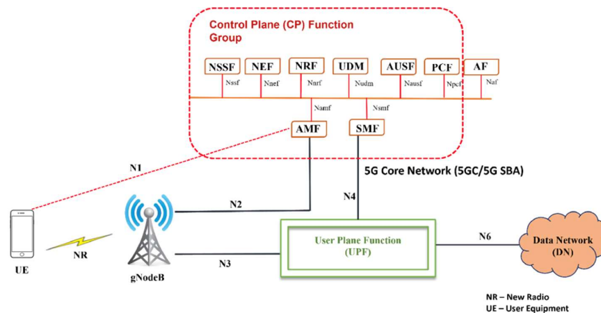
Figure 1: The 5G Generic Architecture
