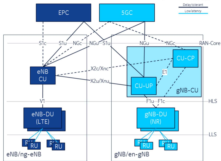
Figure 2: Disaggregated RAN Architecture
