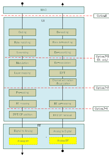
Figure 1: Disaggregated RAN SW Architecture
