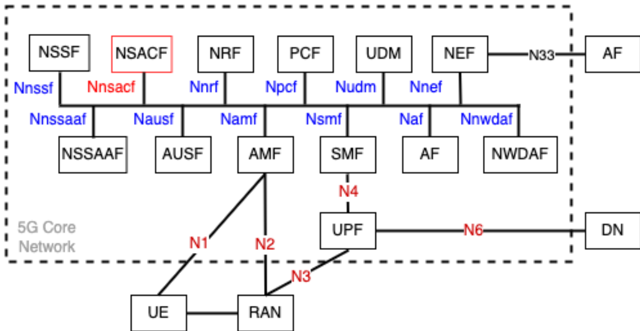
Figure 1: Service based architectural view of 5GS [Adapted from TSDSI STD T1.3GPP 23.501 17.7.0 V1.3.0]
