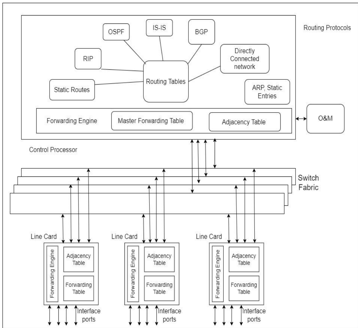
Fig 2: Router Architecture
